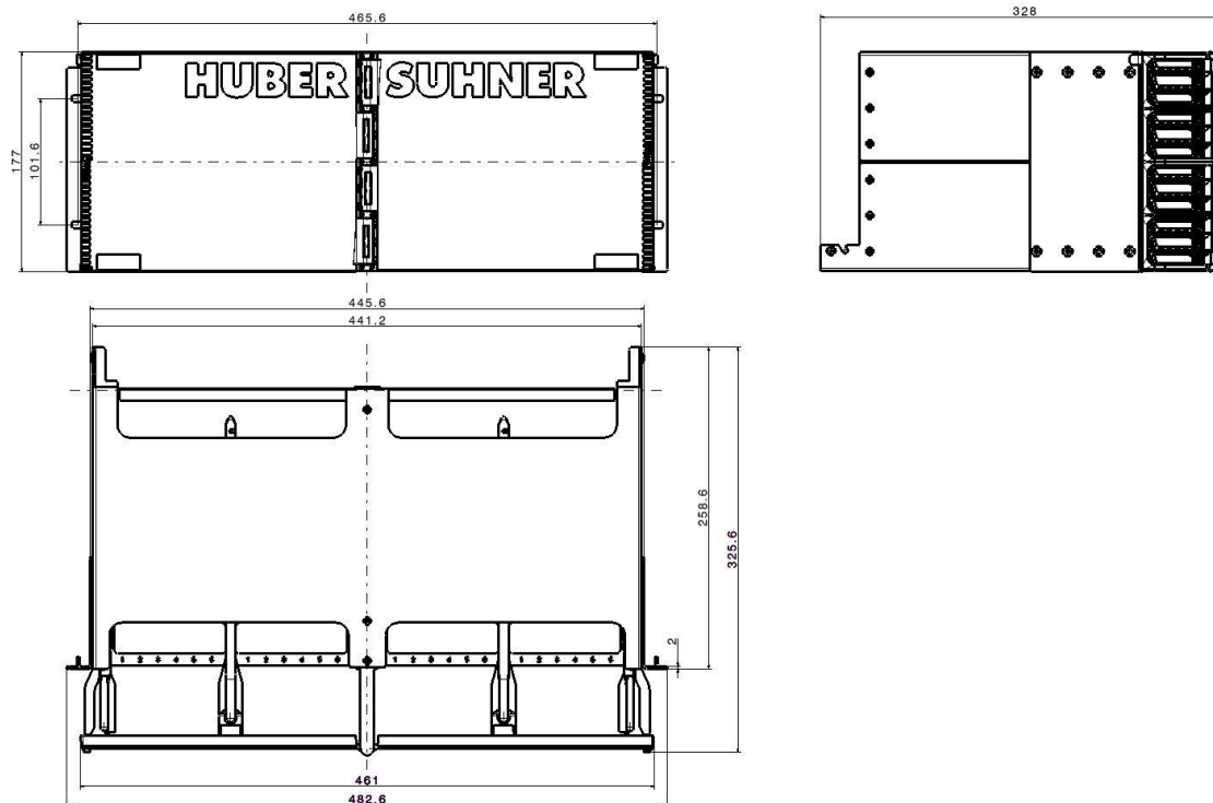
4U Chassis
