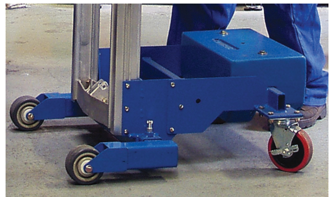
Counterweight Lift has short front legs and rear castors fitted with side brakes.
