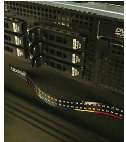
Temperature Strip 46-4000-10009
